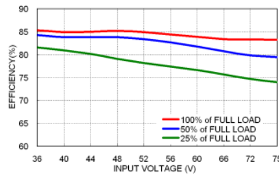
43MPP06-48S05WA Efficiency vs. Input Voltage
