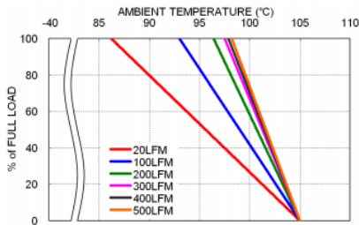
43MPP06-48S05WA Derating Curve
