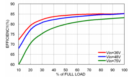
43MPP06-48S05WA Efficiency vs. Output Load
